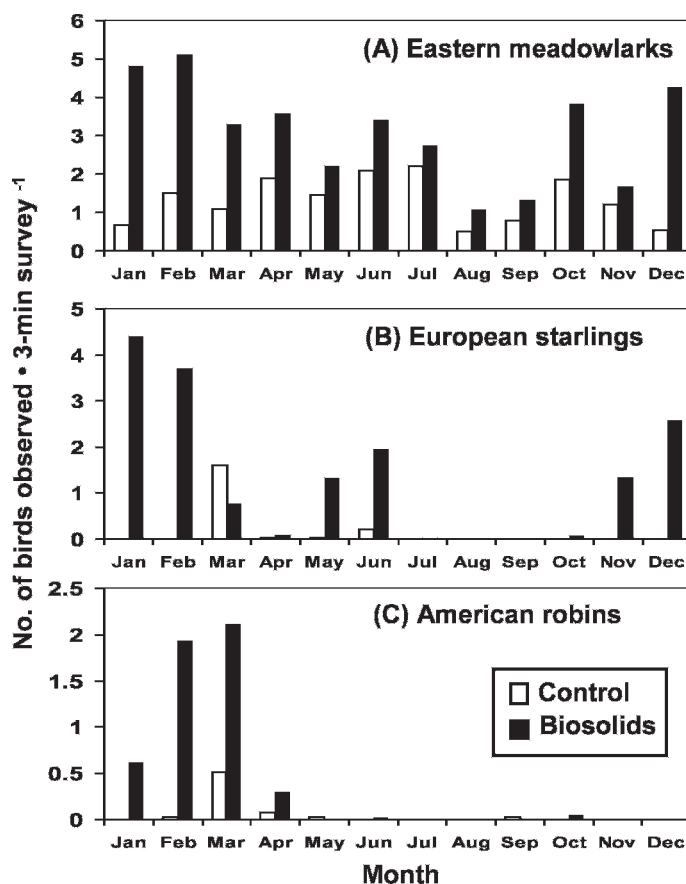
Figure 3. Mean no. of Eastern meadowlarks (A), European starlings (B), and American robins (C) observed \cdot 3-min survey -1 , by month, in control and biosolids-treated monitoring plots at Marine Corps Air Station Cherry Point, Havelock, North Carolina, December 2003 through December 2005.
