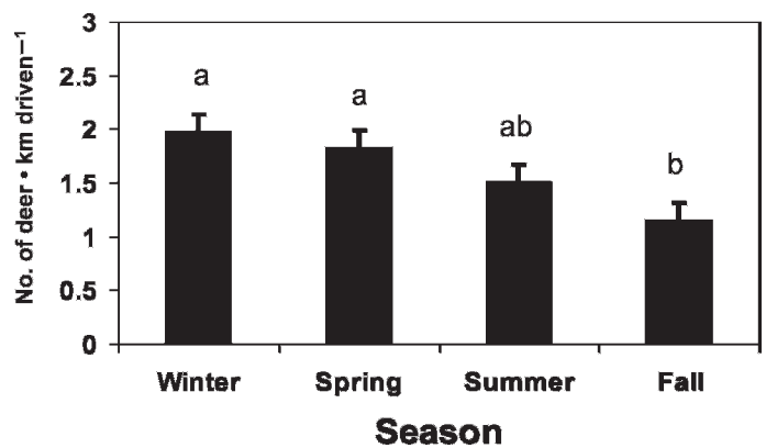
Figure 5. Mean ( \pm SE) no. of white-tailed deer observed \cdot km driven ^{-1} , by season, in grassland areas on the airfield at Marine Corps Air Station Cherry Point, Havelock, North Carolina, 2000–2005. Means with the same letter are not significantly different (Mann–Whitney U-test; P > 0.05 ).
