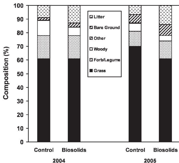
Figure 2. Mean percent cover of plant community characteristics in control and biosolids-treated plots located in grassland habitats on the Marine Corps Air Station Cherry Point airfield, Havelock, North Carolina, during April through September of 2004 and 2005.
